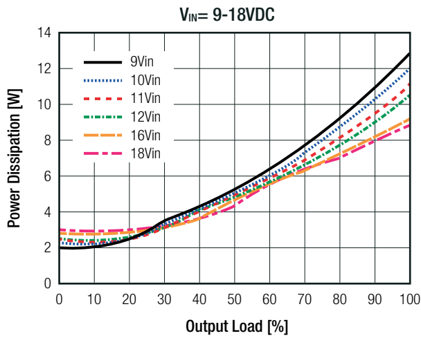
Power Dissipation vs. Output Current
