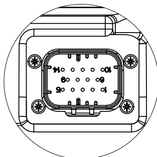
DETAIL CON2
