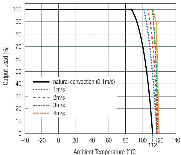
RPMGE5.0-10
