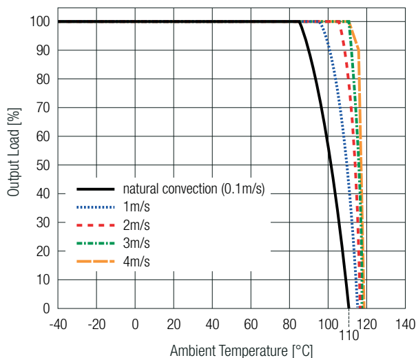
RPMGE12-10
