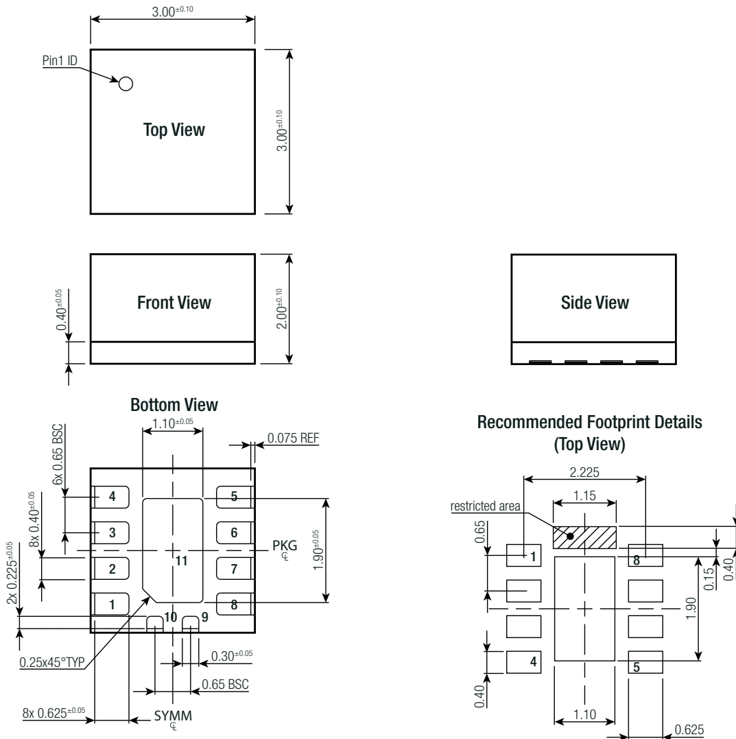
Dimension Drawing (mm)
