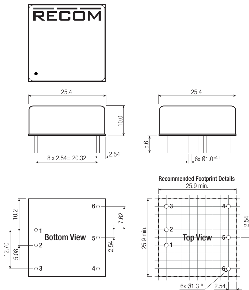
Dimension Drawing (mm)
