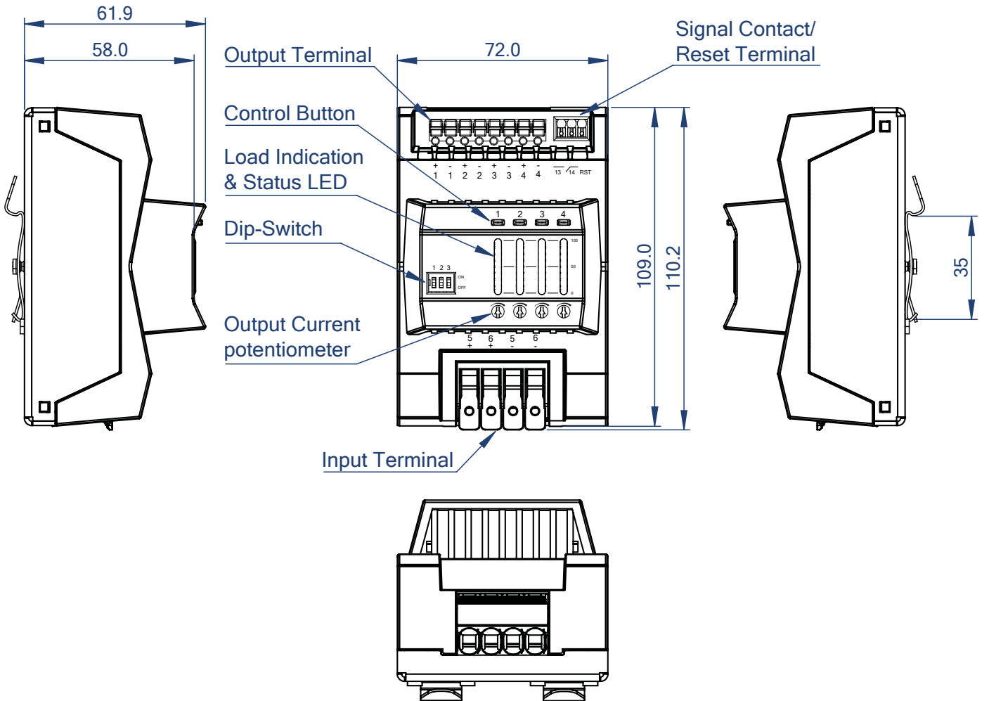
Dimension Drawing (mm)
